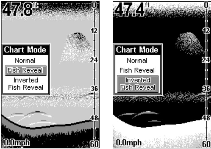
At left, standard FishReveal mode. Right, Inverted Fish Reveal mode.
